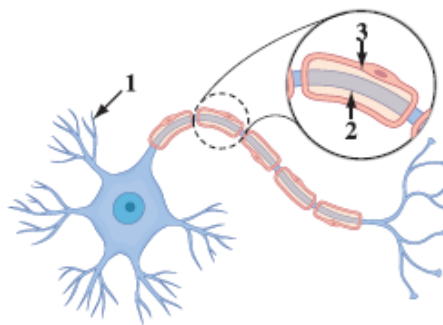
A Neuron
